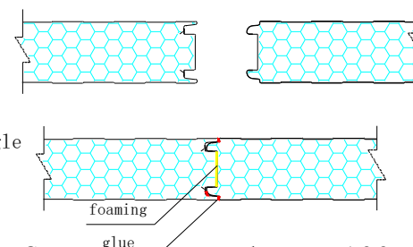
Connection node of 100mm warehouse panels
