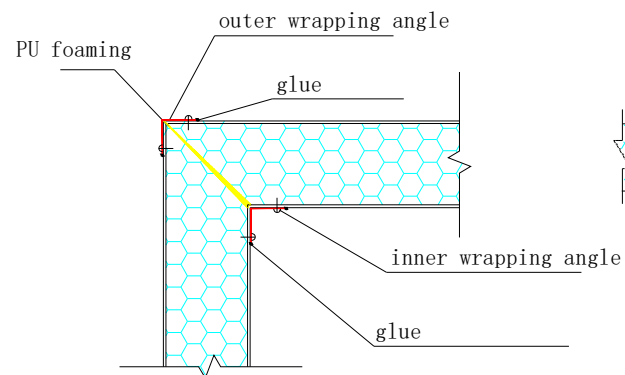
Wall panel corner connection node
