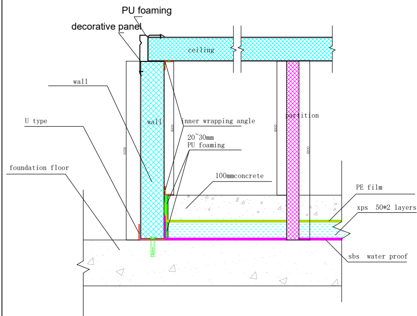
Ground insulation detail drawing
